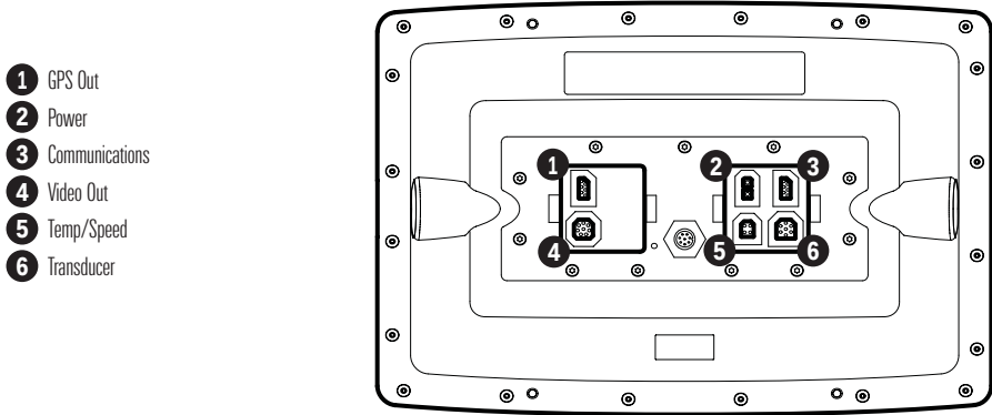
1100 Series™ Connectors
