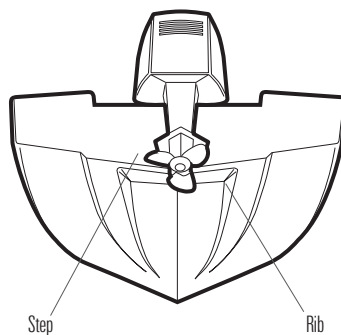
Stepped Hull
